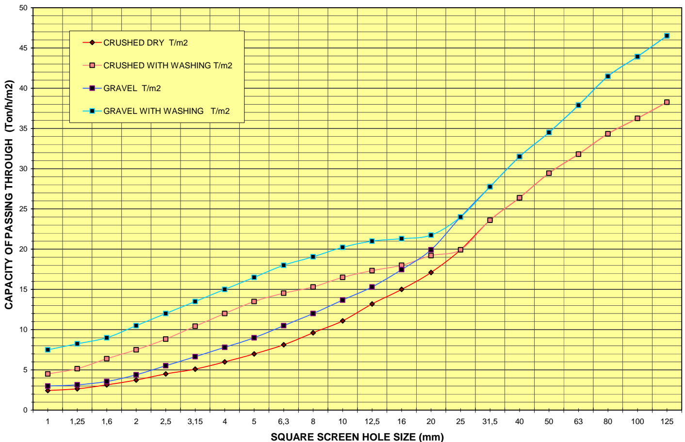
PRODUCT CURVES OF VIBRATING SCREENS mod. "MVI"
