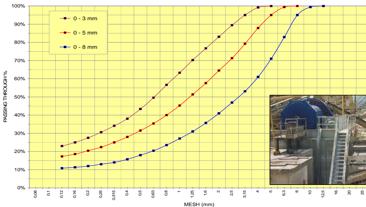
PRODUCT CURVES OF ROD MILLS WITH LATERAL DISCHARGE mod. "MMBL"
