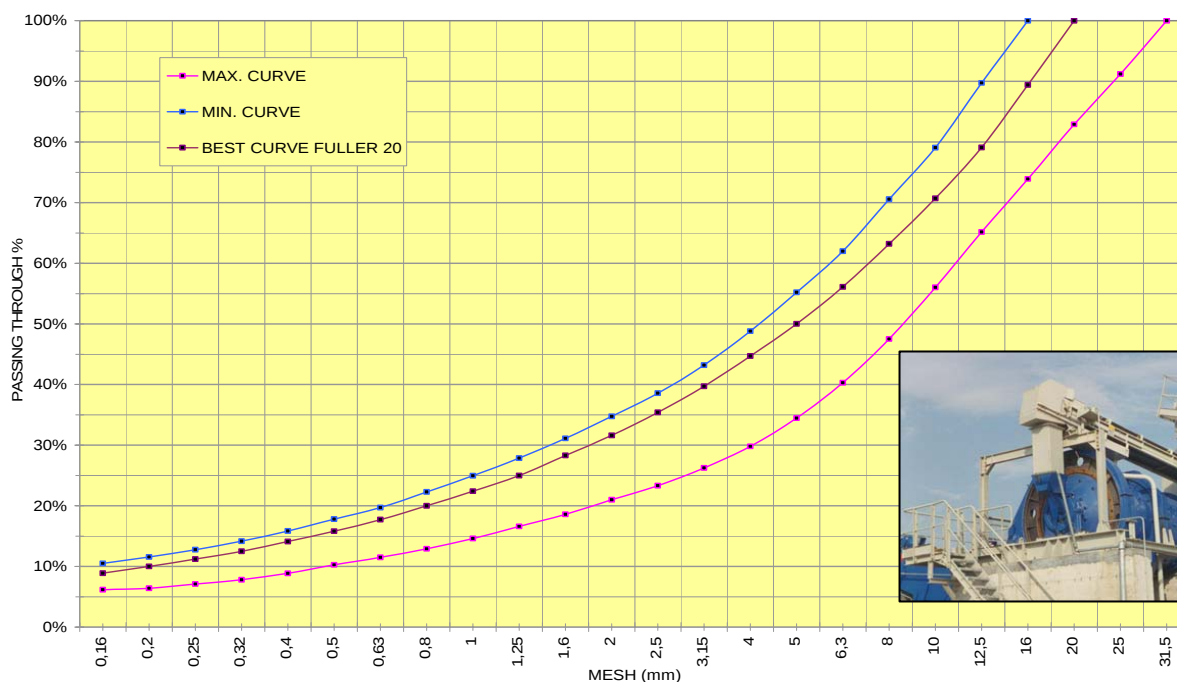
PRODUCT CURVES OF ROD MILLS WITH CENTRAL DISCHARGE mod. "MMBC"
